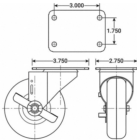
Mounting Plate Bolt Hole Pattern D Mounting Hole Diameter: 5/16"
